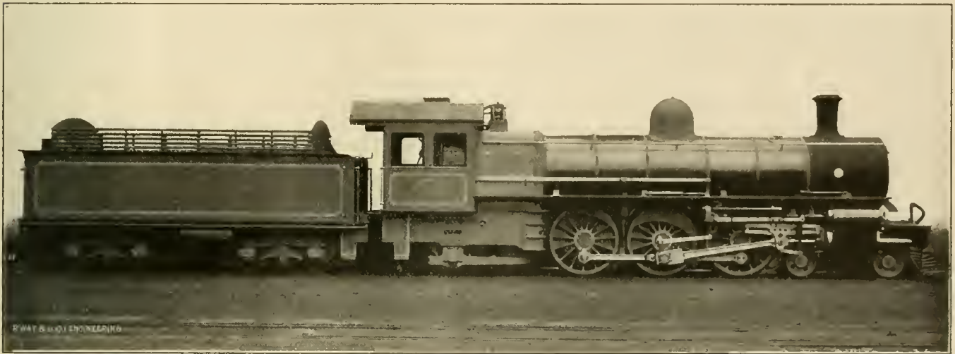
CENTRAL SOUTH AFRICAN 4-6-2 ENGINE WITH WALSCHÄERT VALVE, GEAR.
